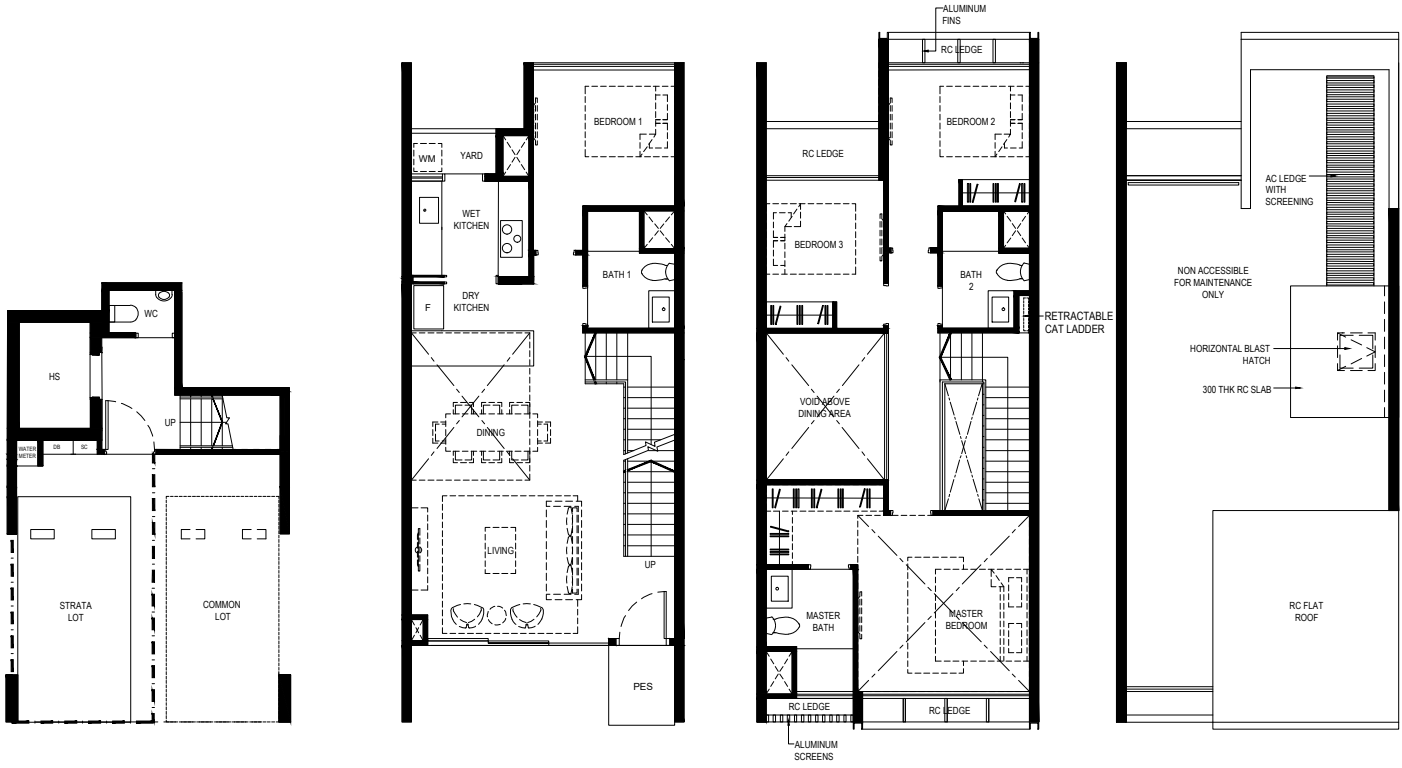
Basement 1
